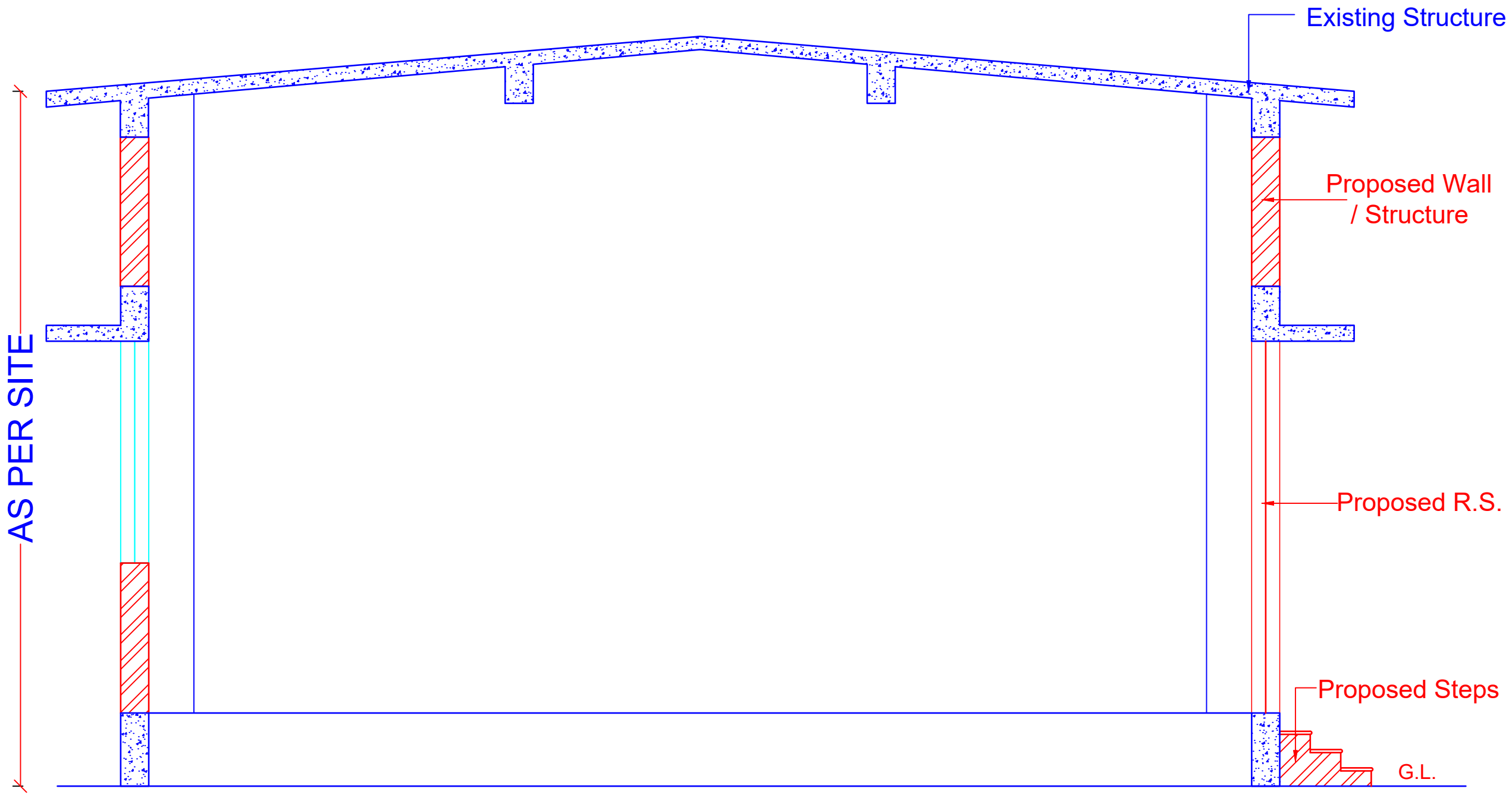
SECTION A—A'
