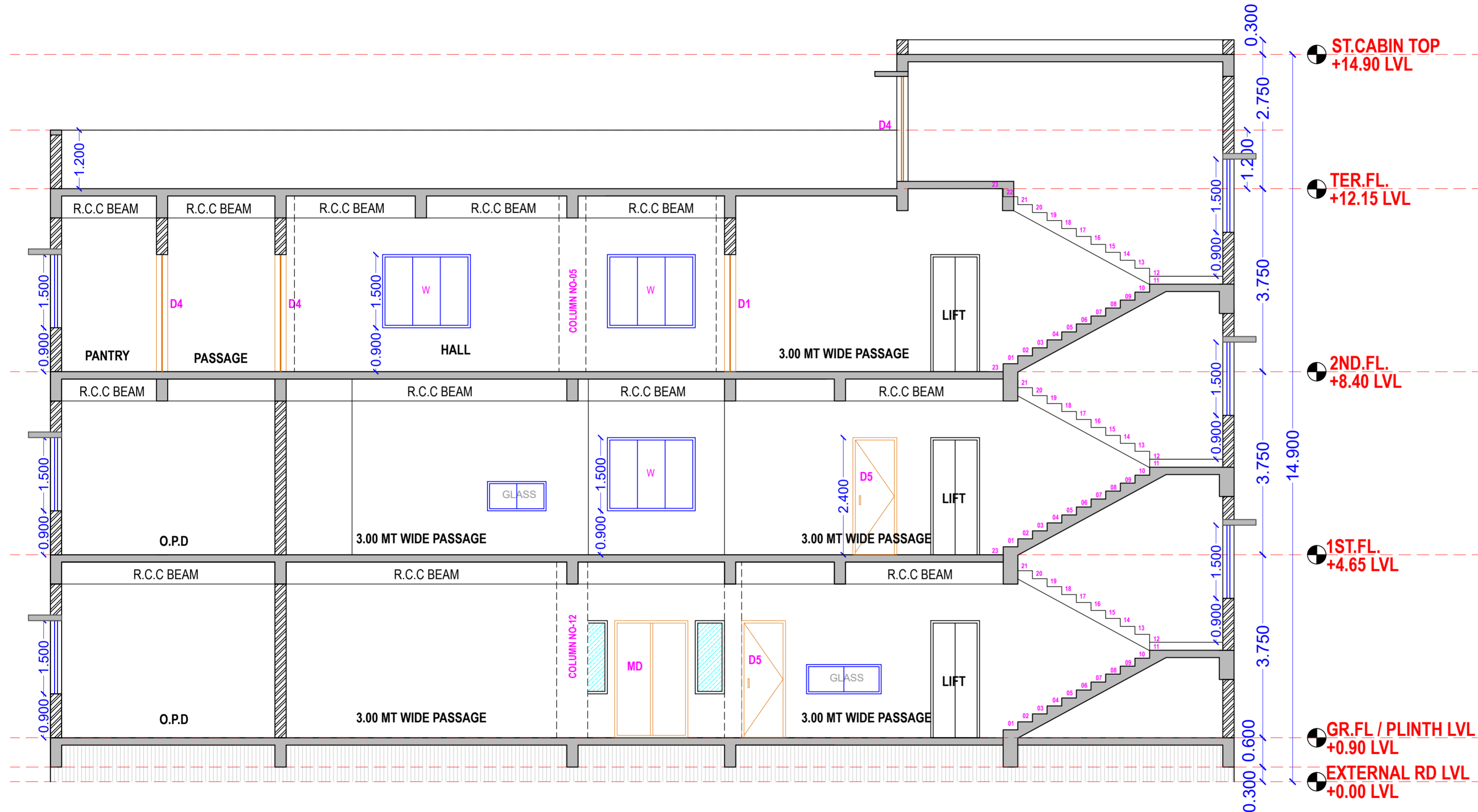
SECTION AA'
