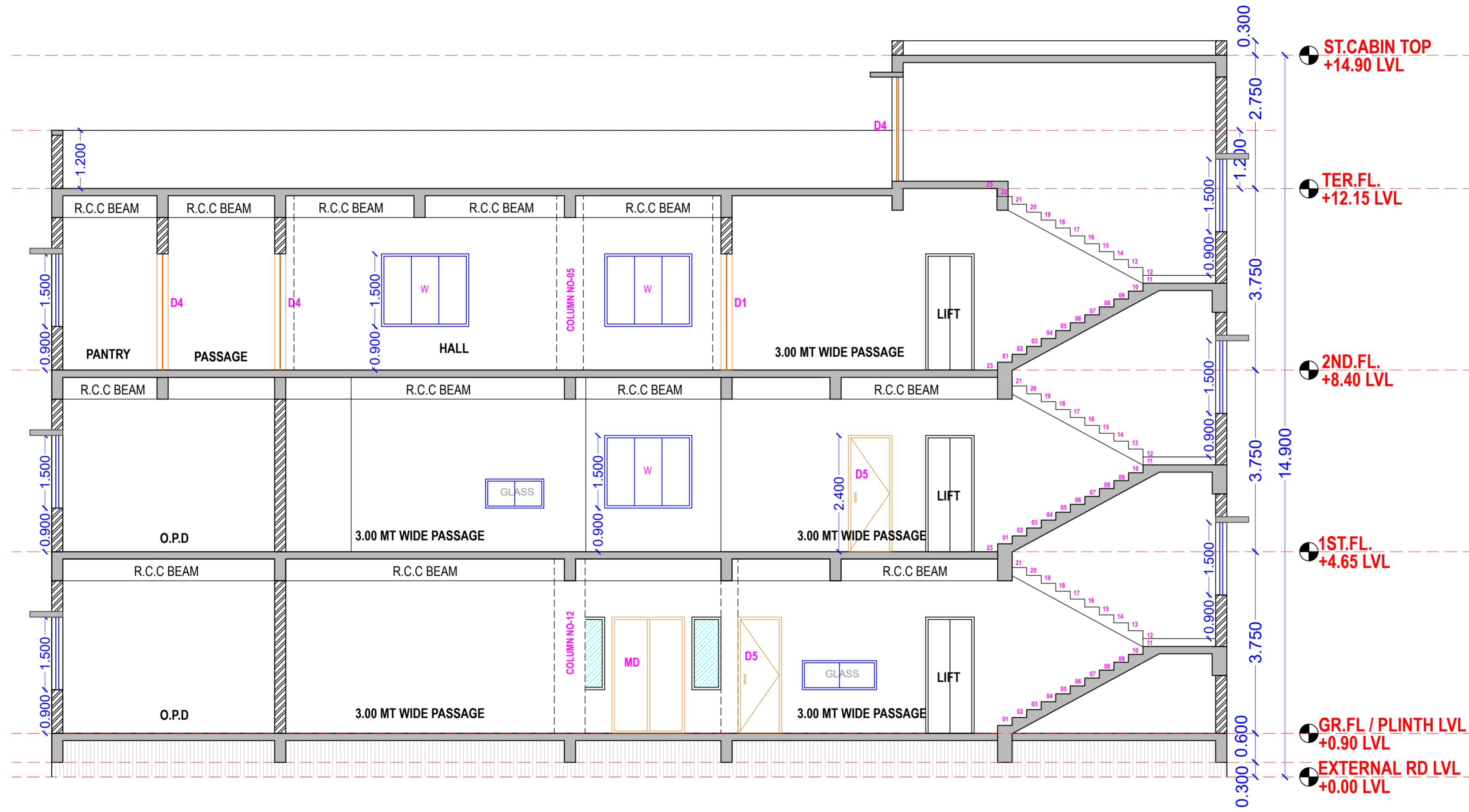
SECTION AA'
