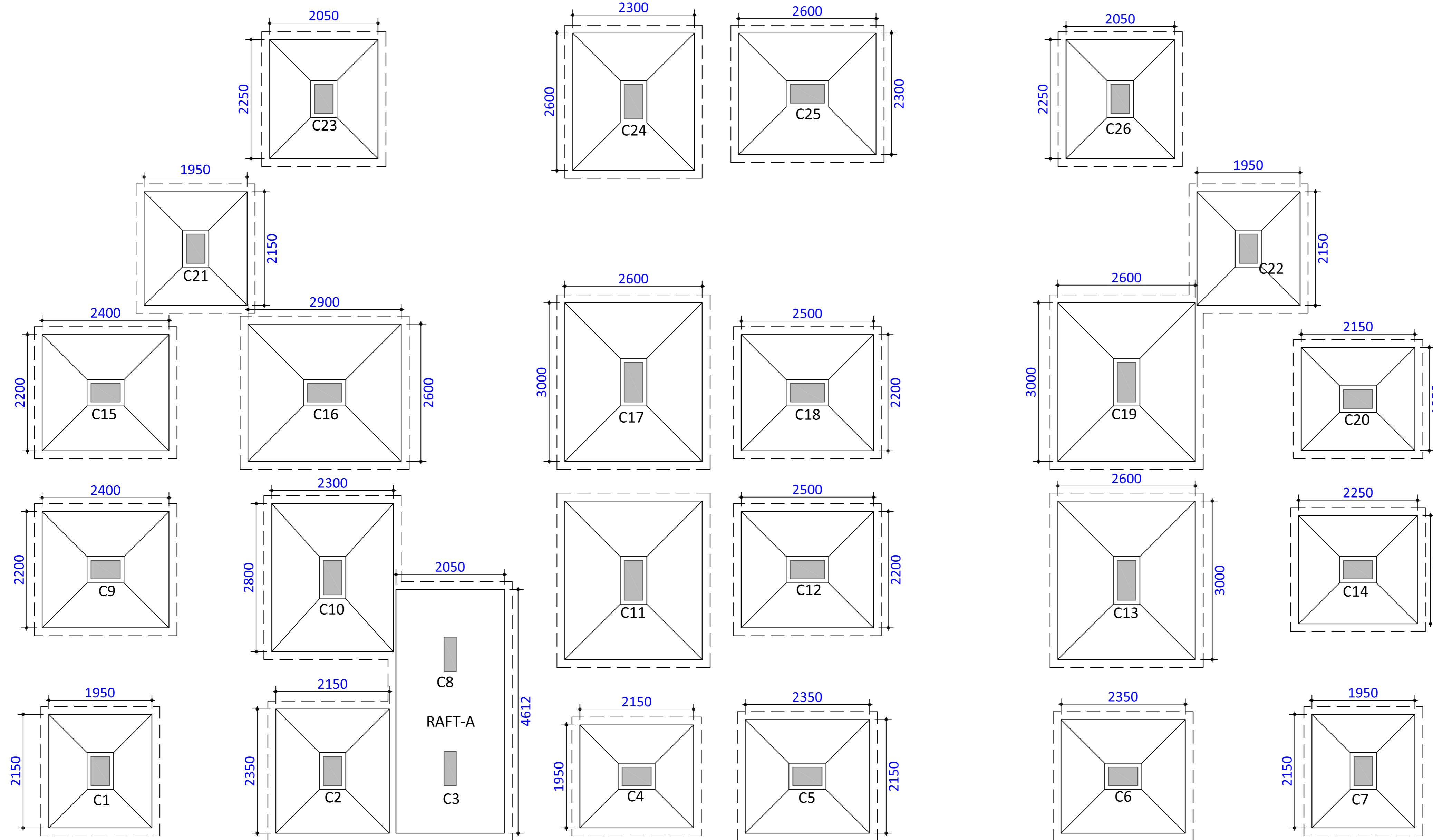
FOOTING LAYOUT
