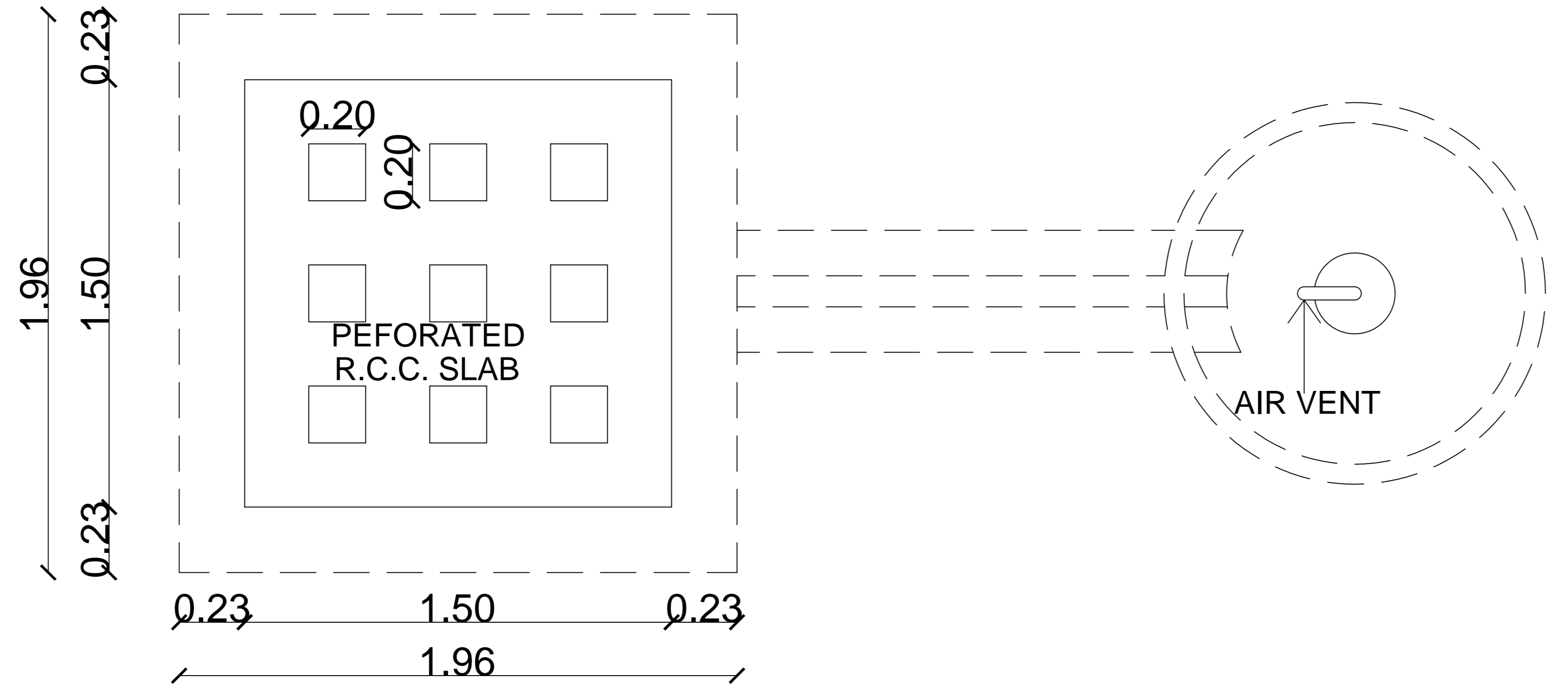
BOREHOLE FOR WATER HARVESTING SYSTEM PLAN
