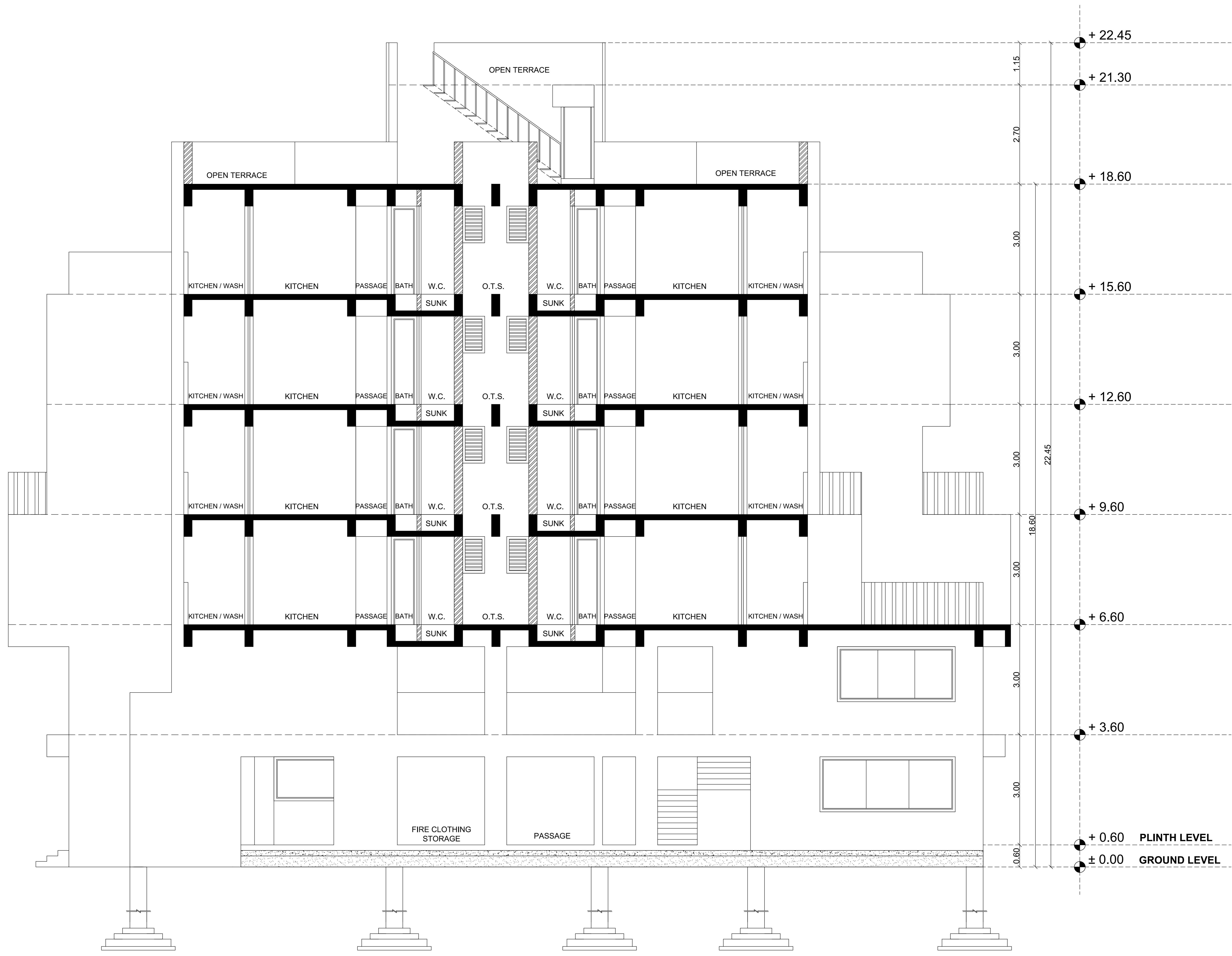
SECTION- B-B''
