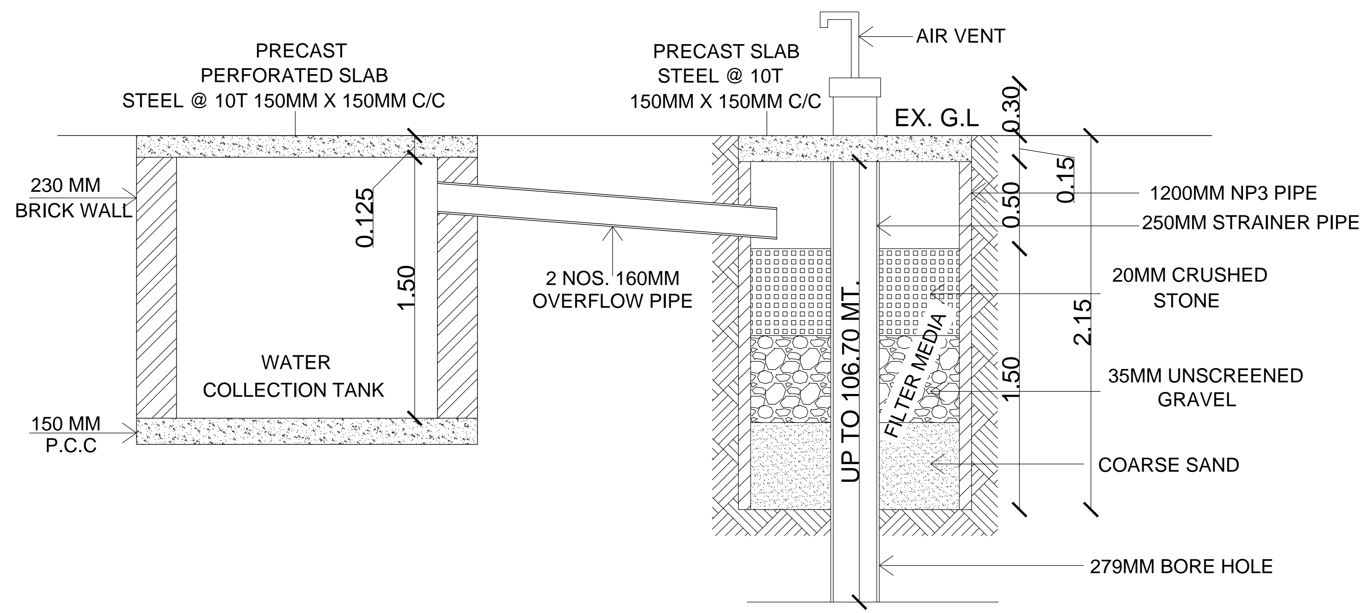
BOREHOLE FOR WATER HARVESTING SYSTEM SECTION
