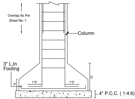
Sectional Elevation
