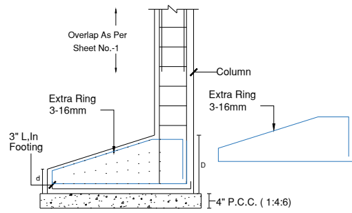
Sectional Elevation
